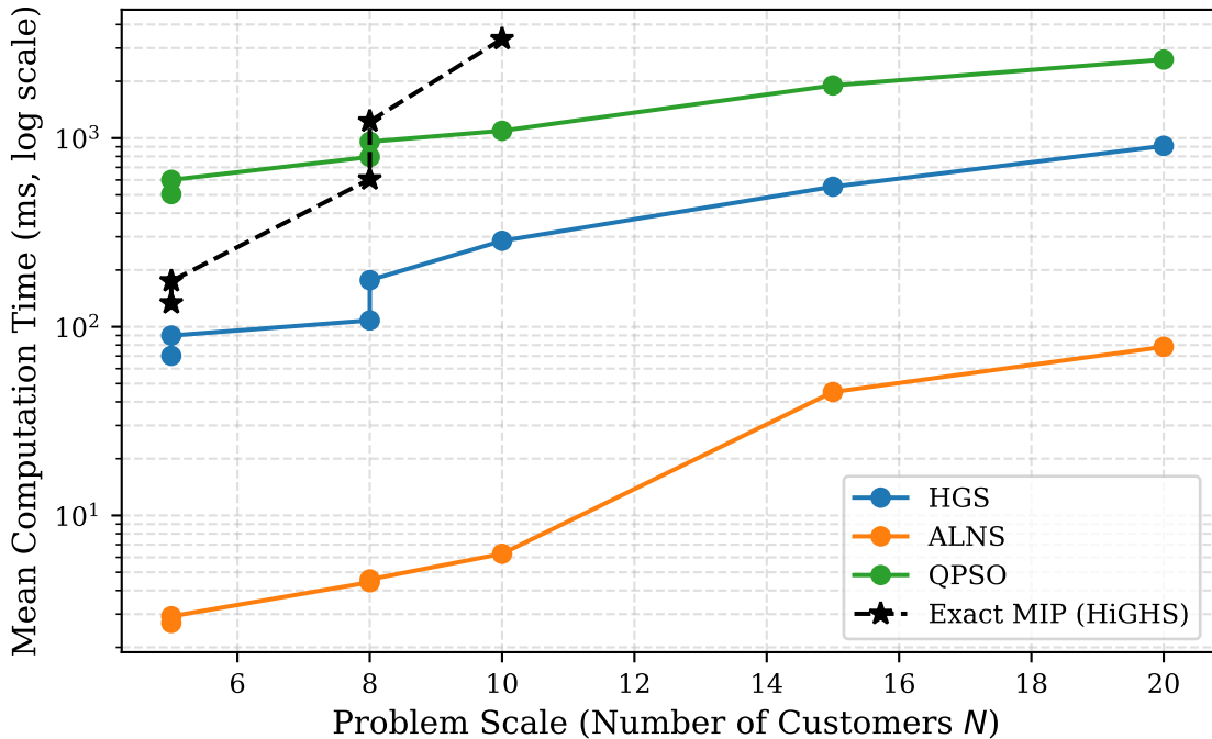
Algorithmic Runtime Scaling Under Equal Evaluation Budget
